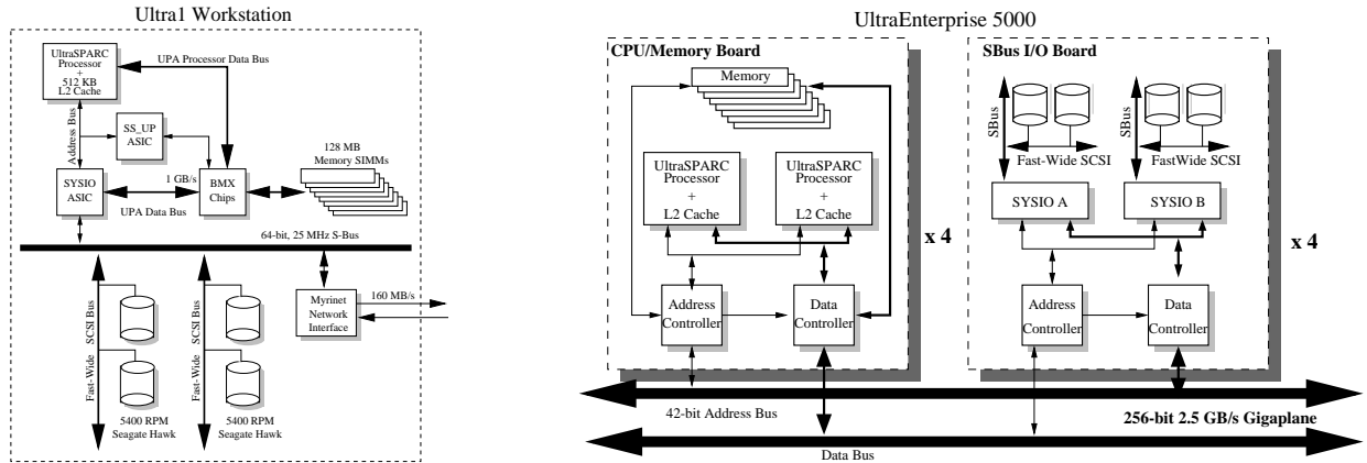
Figure 1: Hardware Diagram. This figure depicts the internals of an Ultra 1 workstation and the Ultra Enterprise 5000. Workstation: Inside the workstation on the left, the BMX crossbar chips and SS_L/P ASIC controller provide switched-based access to memory. SMP: On the right is the Enterprise 5000. Each CPU board houses two CPUs, which share an address and a data bus. Each I/O board consists of two S-Bus I/O busses. All boards are connected to the main memory interconnect (GigaPlane). Though memory is physically distributed, access time is uniform.
